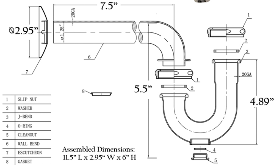
Shown without tailpipe *for use with Victorian Sinks/Vanity Drain
